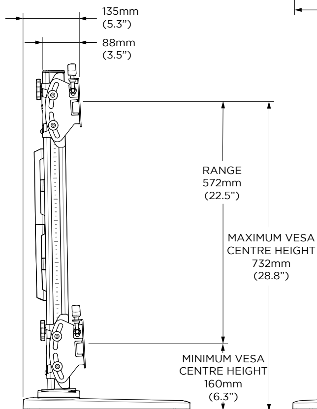
SIDE VIEW
